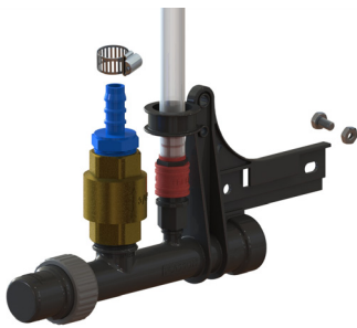
02204041 Modular Line End Detachable Sight Tube 3/4" BSPT W/Non- Return Valve COM.
